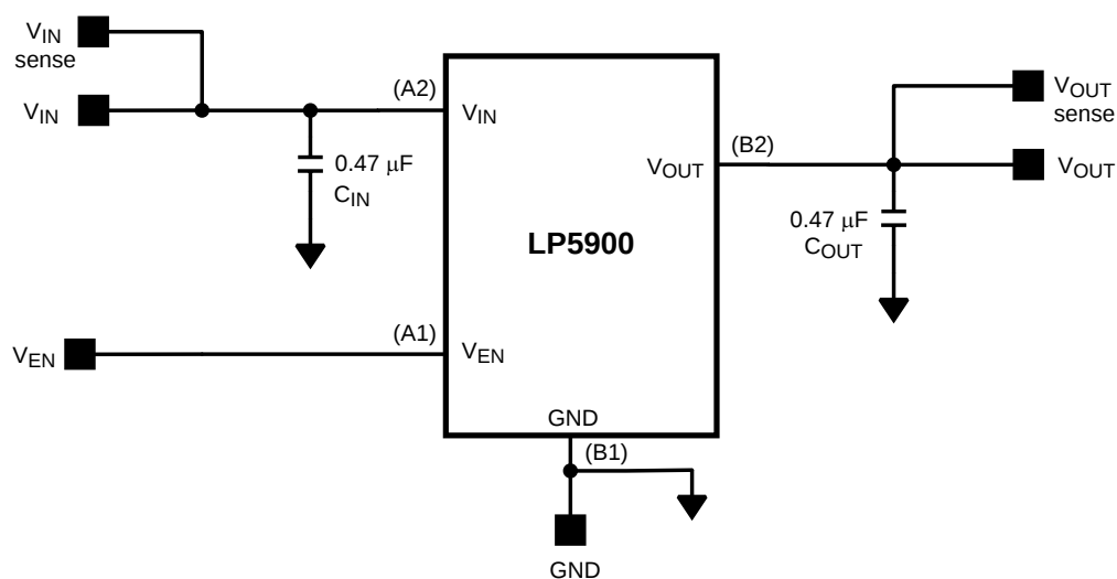
Figure 1. Evaluation Board Schematic
